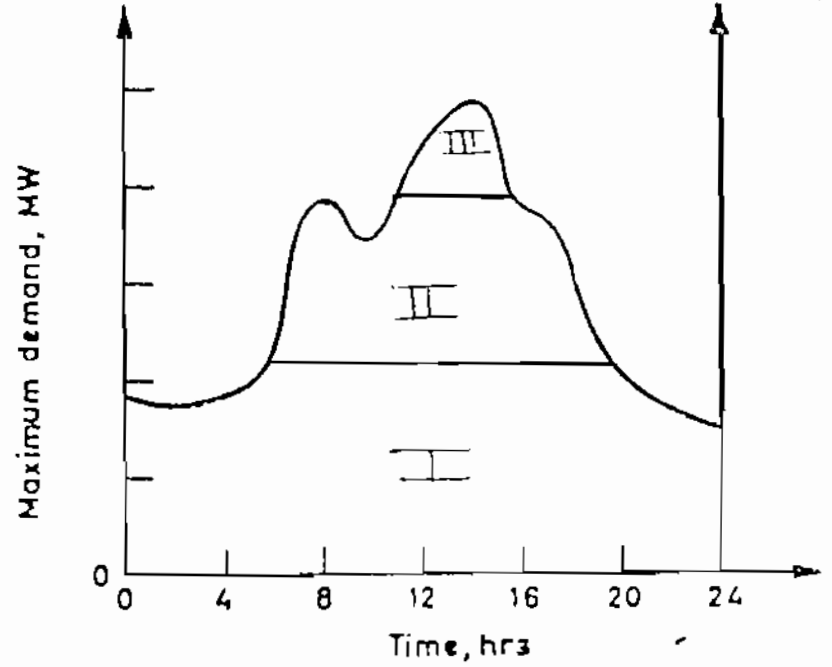
Typical daily load curve
