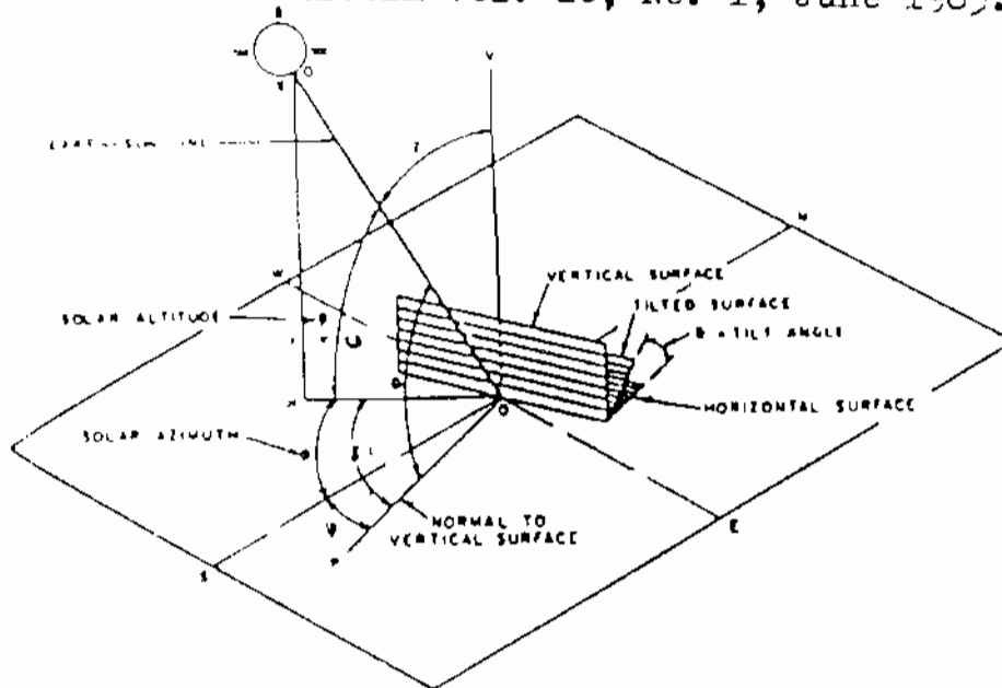
Fig (5,b) Solar Angles For Vertical And Horizontal Surfaces.
