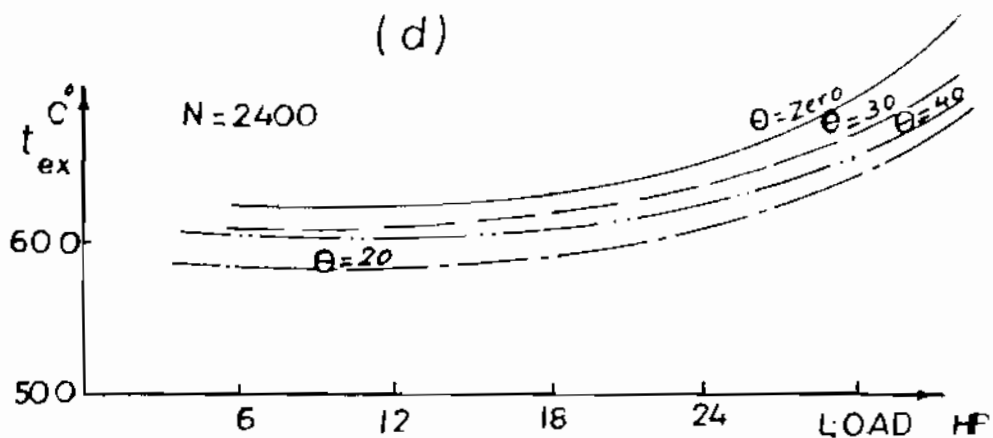
Fig.(9) Relations of exhaust gas temperature
