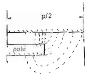
Fig. (9) : Quadrature axis flux distribution
