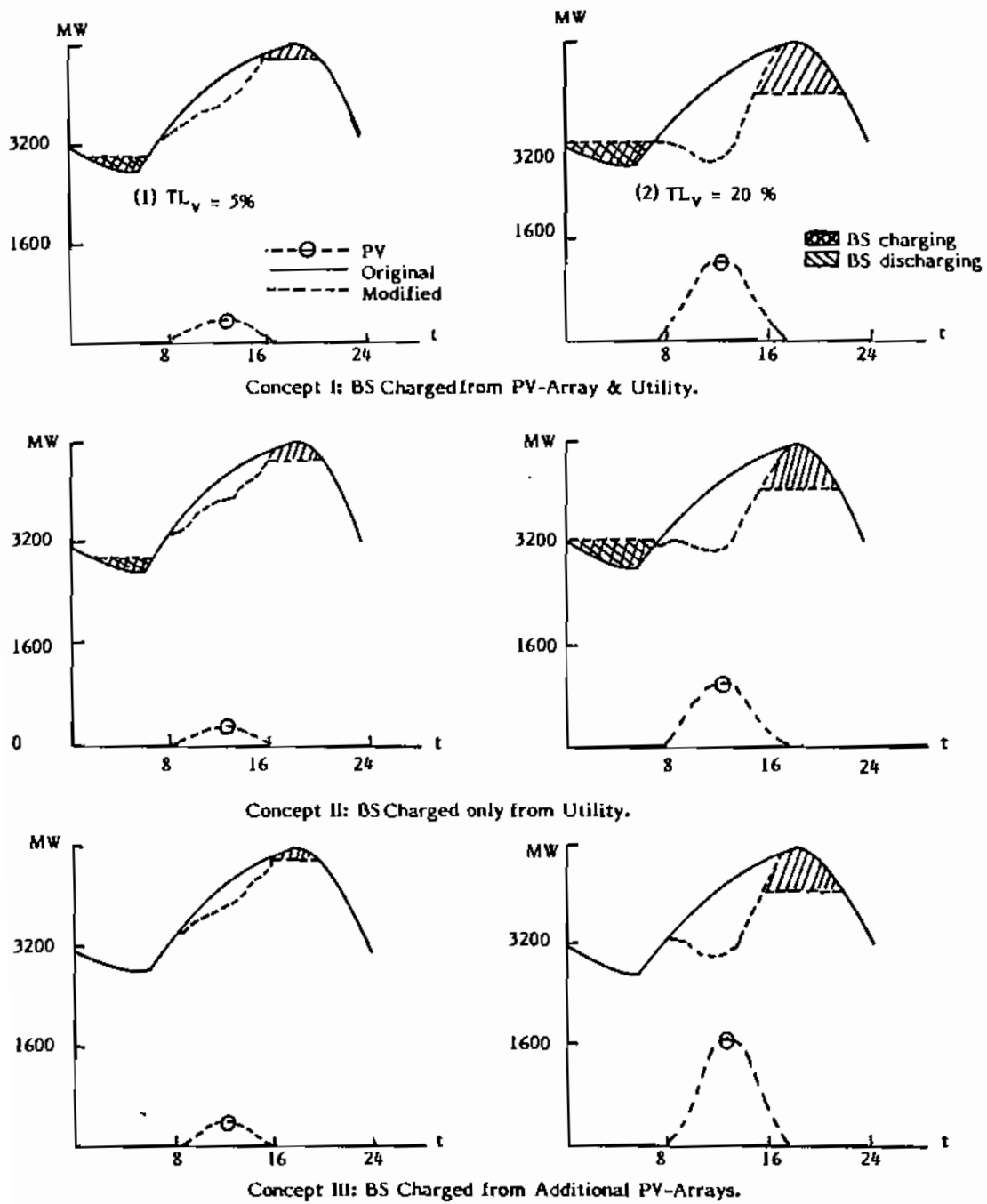
Fig. 3-b PV and Original & Modified Average Daily Conventional Generation Curves Applying the Proposed Design Concepts I, II & III, (January, Winter).
