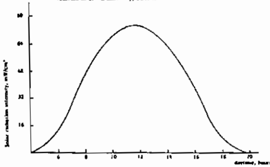
Fig. 12-b Actual daily solar radiation intensity pattern of summer season (July) recorded at El-Mansoura city, EGYPT.
