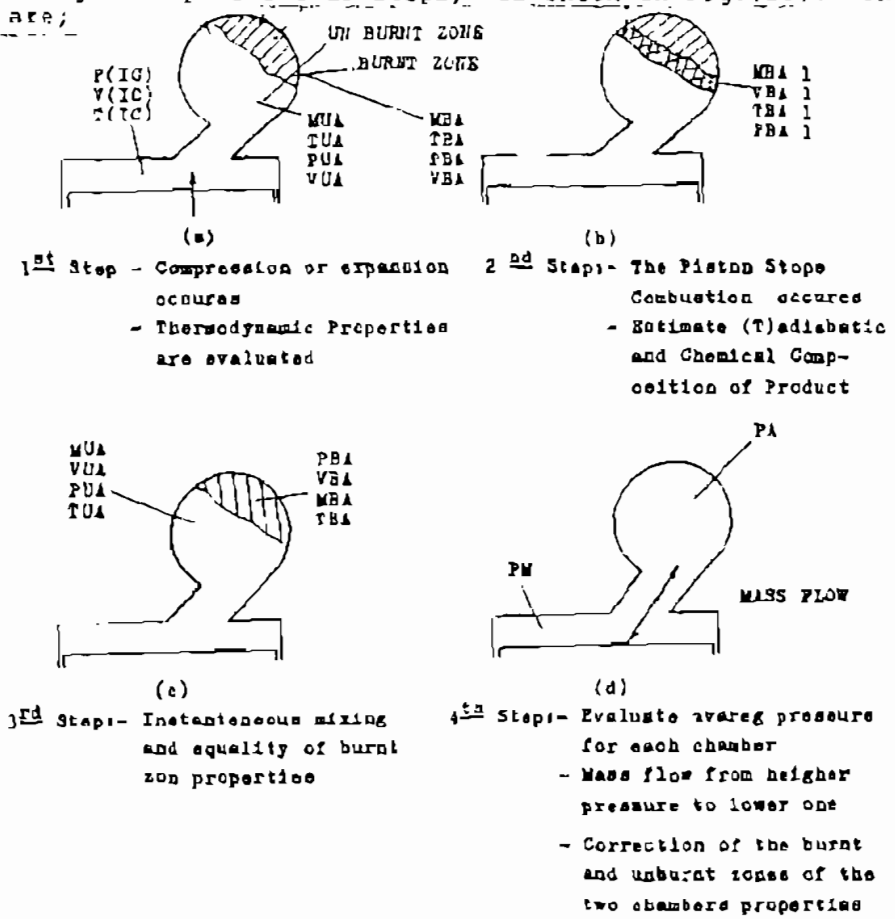
Fig. (16) Analysis Of Combustion Process where; MUA, TUA, PUA and VUA are mass, temperature, pressure and volume of unburnt gas in the prechamber, MBA, TBA, PBA and VBA are mass temperature, pressure and volume of burnt gas,
