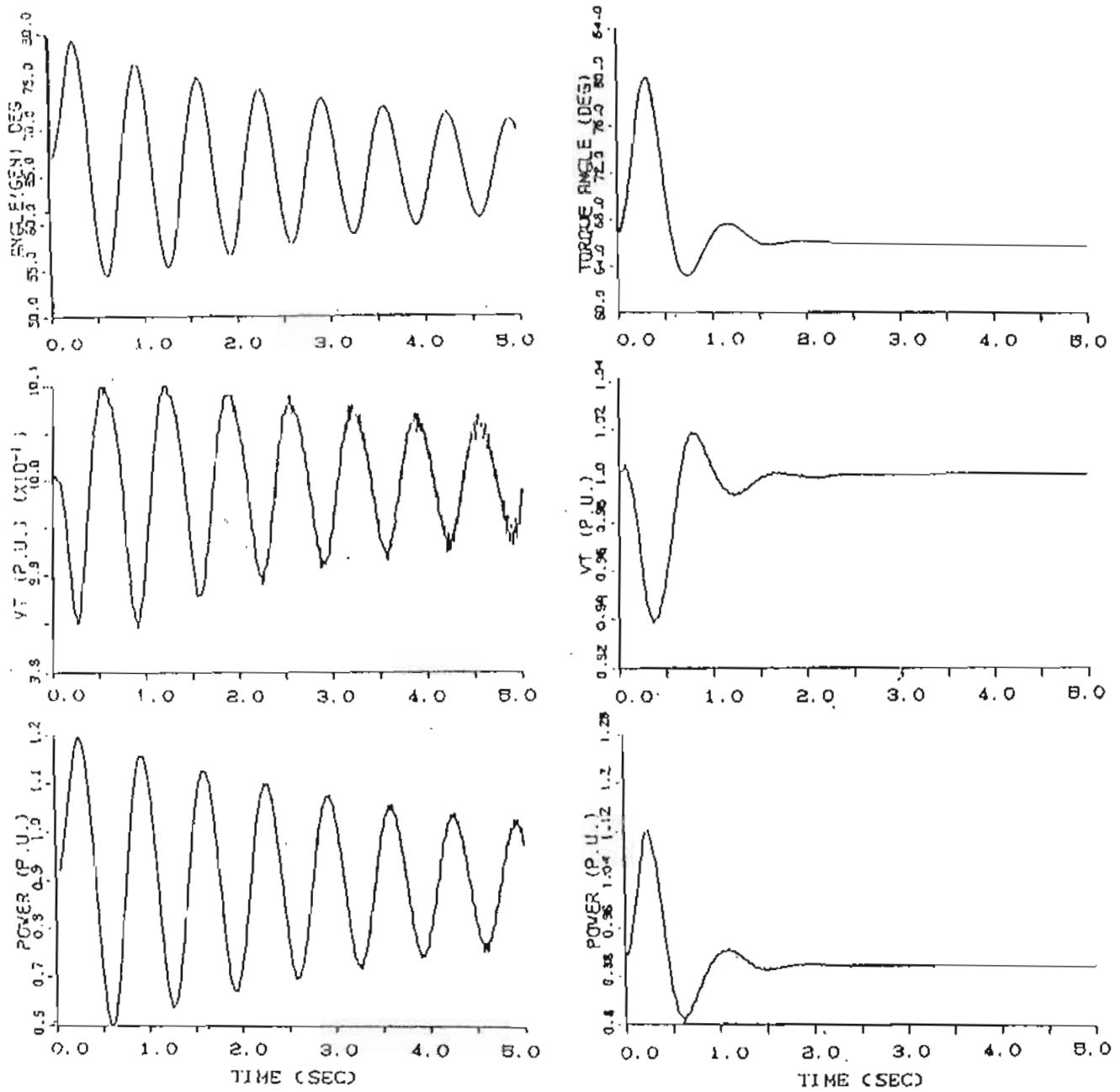
Figure 1 Dynamic response of the generator (left) without control; (right) with control
