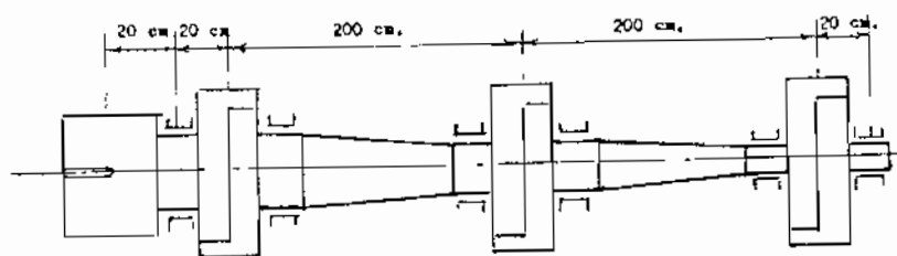
Figure(8) Device of Stepped-Taper One Driving Shaft.
