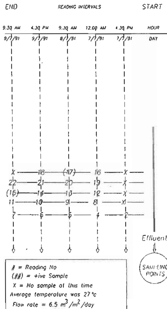
Slow Sand Filter #2
