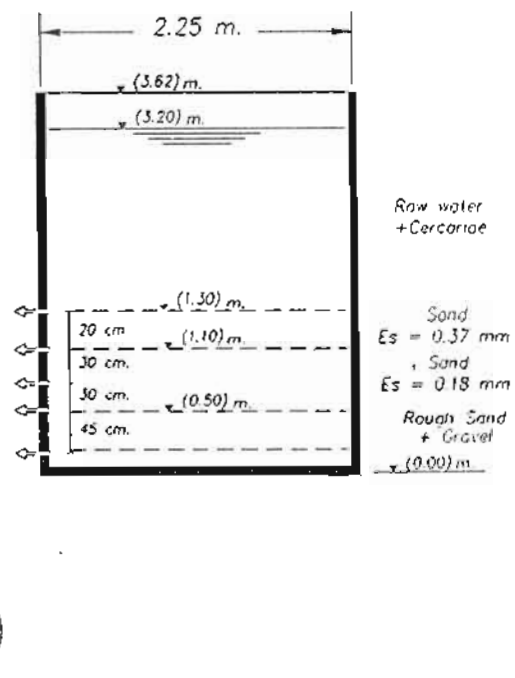
Slow Sand Filter #2
