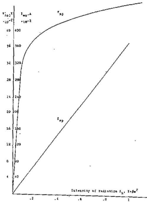
Fig. 2 current and voltage at a maximum power points of a solar cell at 433Kev/m 2 insolation levels.
