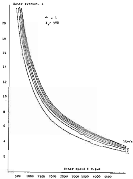
Fig.9 Motor current speed characteristics for different insulation levels, \mu=1 and number of connected series cells, Z_p = 500 .
