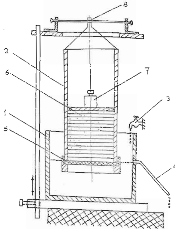
Fig. 1. An Apparatus For Testing Absorbability of Felt Fabrics
