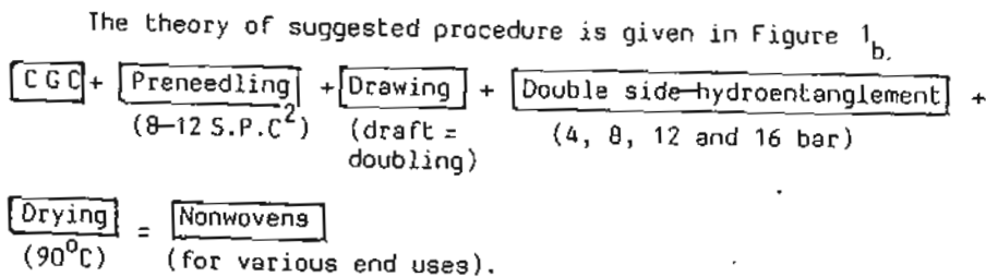
Fig. 1: Shows the principles of preneedling, drawing, and hydroentanglement procedure.
