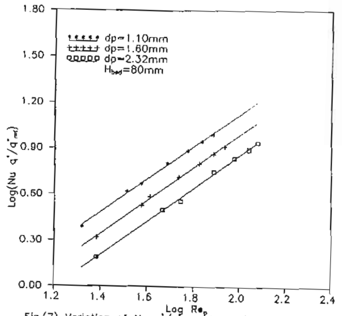
Fig.(7) Variation of Nu q'/q'_{mf} with particle Reynolds number ( Re_p ) for different bed diameter.
