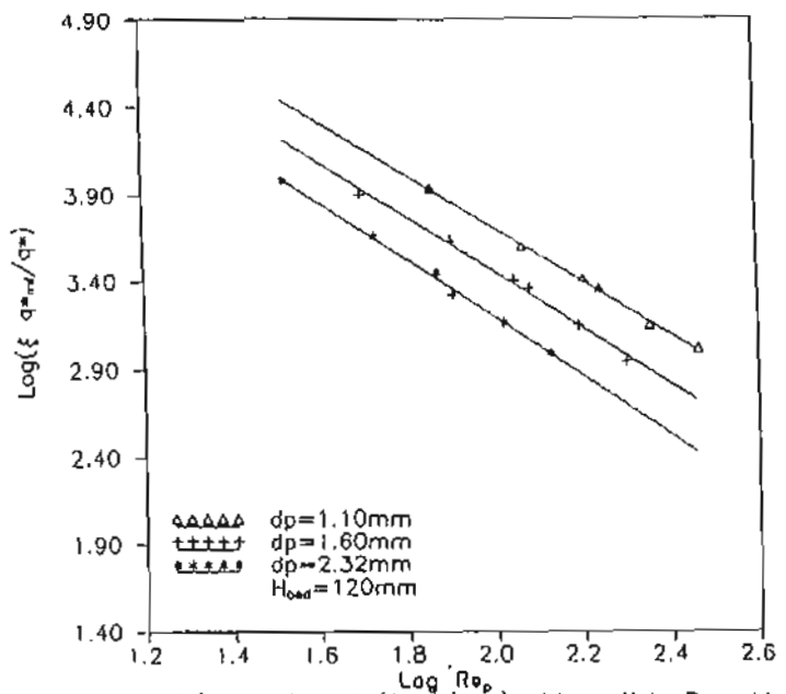
Fig.(4) Variation of (\xi q^*/q_{*mi}^*) with particle Reynolds number ( Re_p ) for different bed diameter.
