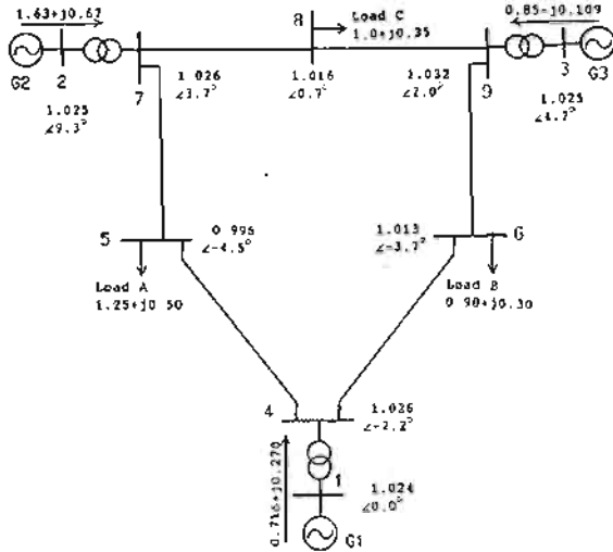
Fig.1 Power System # 1
