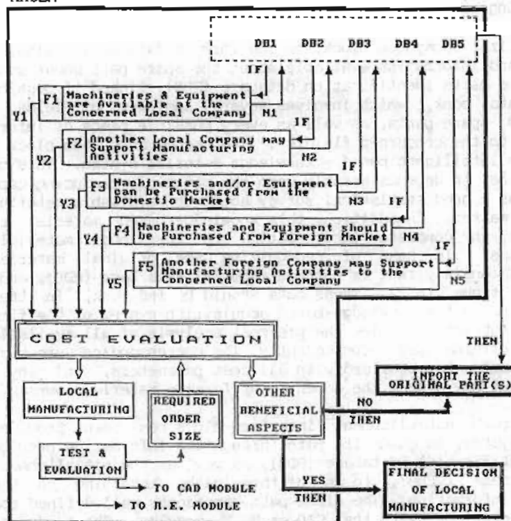
Fig.4 Image of the Expert Cost Analysis Subsystem.
