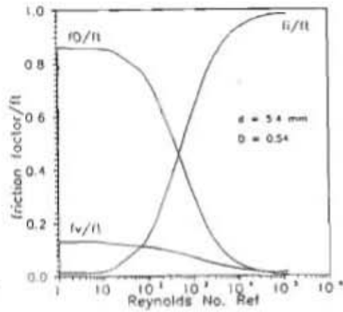
Fig.12 friction factors f_D/f_l , f_v/f_l and f_l/f_l variation with Re_f for d=5.4 mm and D=0.54
