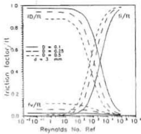
Fig. 11 friction factors f_D/f_l , f_v/f_l and f_l/f_l variation with Re_f for d=3 mm and D=0.1
