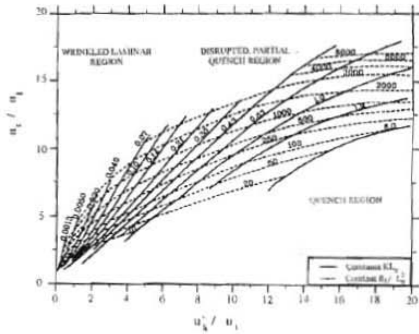
Fig. 1 The relationship between u' / u_1 and u'' / u_1 suggested by the Leeds turbulent burning velocity correlations
