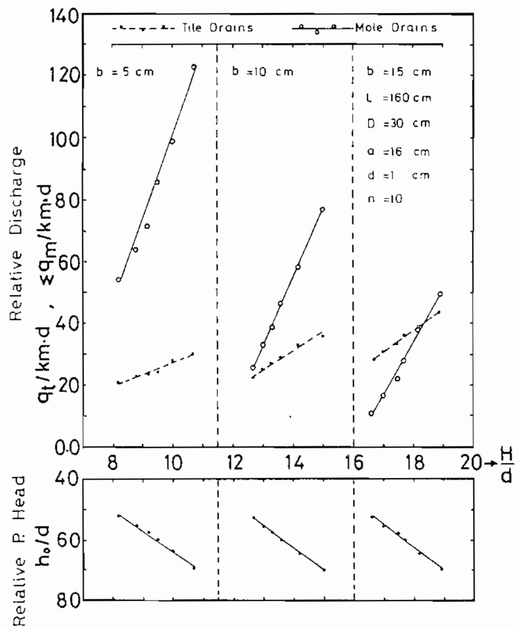
Fig( 4 ) Variation of Relative Discharge and Relative Piezometric Head versus Relative Head( \frac{h}{H} ).
