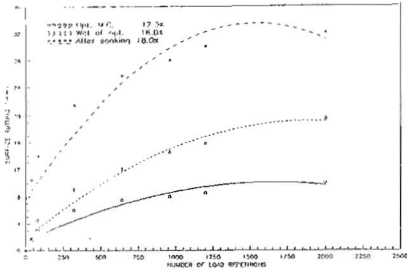
Figure (2) Effect of Subgrade Moisture Content on Progressive Surface Rutting , Witout Reinforcement ( Base Course = 50 Mm )
