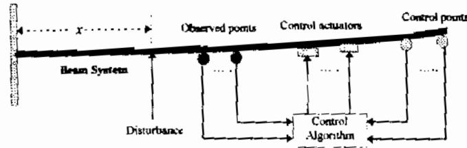
Figure 1. Schematic diagram of the active control system
