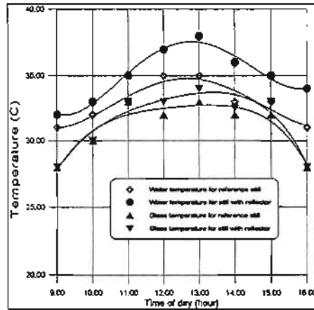
Fig. 4 Variation of temperature during the day 16/9/1998
