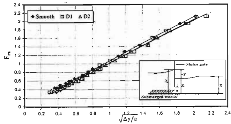
Fig. (17) Relationship between ( F_{ra} ) and \sqrt{\Delta y/a} for the smooth case and the two weeds densities
