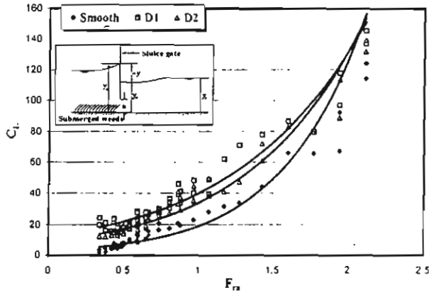
Fig. (20) Relationship between ( C_D ) and ( F_{ra} ) for the smooth case and the two weeds densities
