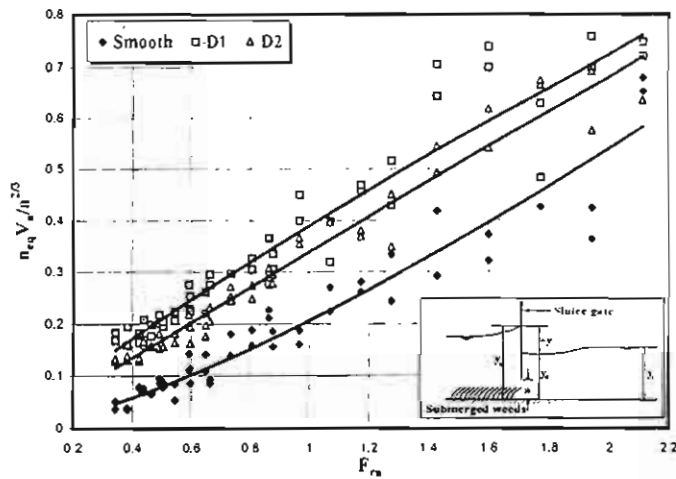
Fig. (25) Relationship between (n_{eq} V_s / a^{2/3}) and (F_{rs}) for the smooth case and the two weeds densities
