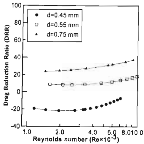
Fig. (18) Effect of diameter on drag reduction ratio at 10 ppm coccentration.
