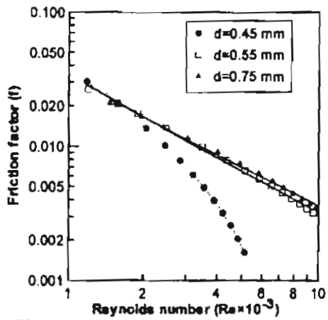
Fig. (6) Friction factor versus Reynolds number at different sizes. (concentration 100 ppm)
