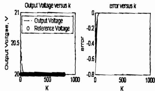
Figure 9. Applying the Adaptive Fuzzy Controller for Case A at time, 2 ms.
