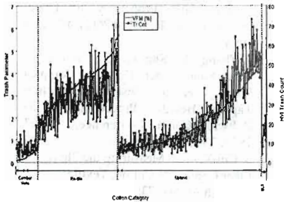
Figure 14. AFIS VFM and HVI Trash Count of all Cottons Excluding Inters
