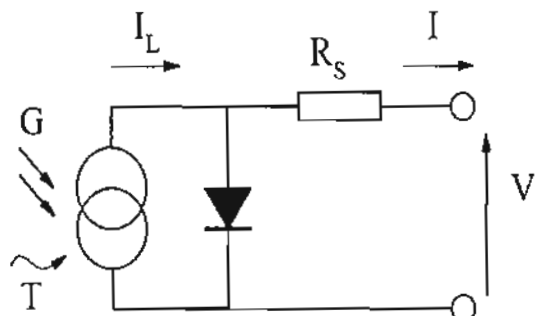
Figure 2: The circuit diagram of the PV model.
