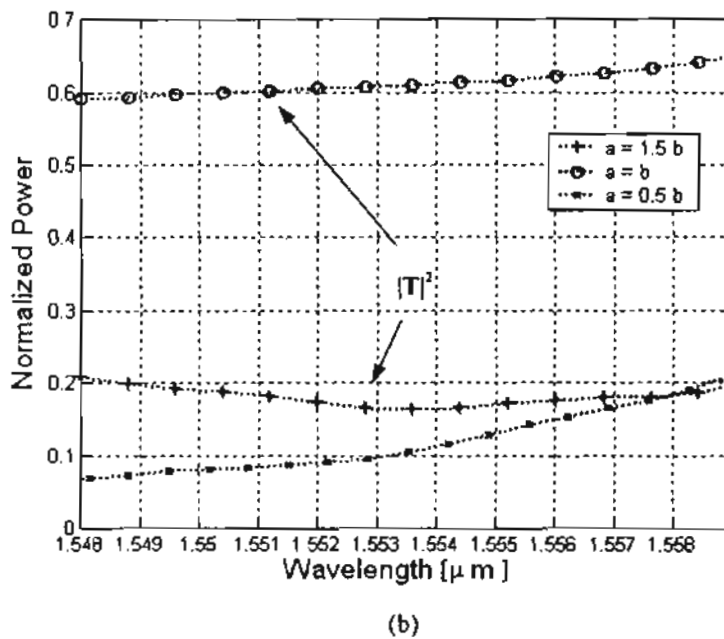
Fig. 10. photonic crystal Ring Resonator of dielectric rods in air : (a) steady state field profile at \lambda = 1.55\mu\text{m} for: Case 1: a=0.5 \times b , b = 5.8\mu\text{m} , Case 2: a = b = 5.8\mu\text{m} and Case 3: a = 1.5 \times b , b = 5.8 \mu\text{m} , (b) The transmitted power to the drop channel.
