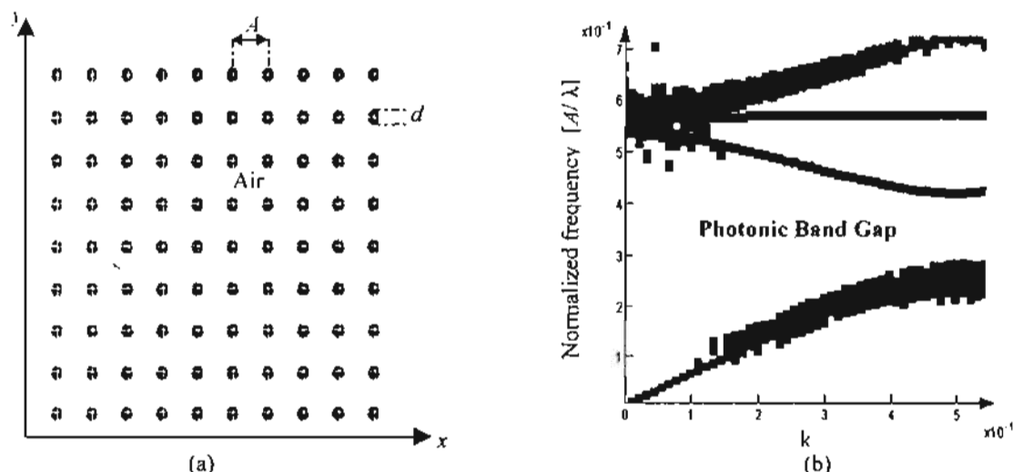
Fig. 5. Cross section of square lattice of dielectric rods arranged in air: (a) Details of the structure A = 0.58 \mu\text{m} , d = .36A , n = 3.4 , (b) Calculated band structure for TE mode.
