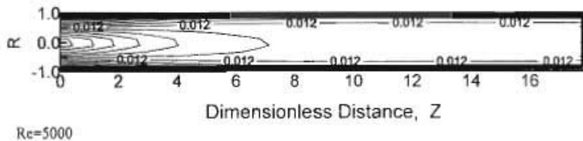
Figure (5) Iso-mass lines for different Reynolds number
