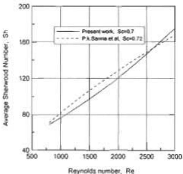
Fig (7) Comparison between Average Sherwood number
