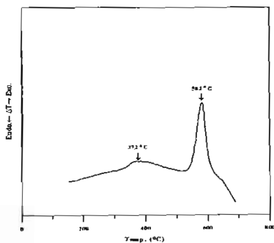
Fig. 6: DTA curve of 40 h milled powder for \text{Al}_{86}\text{Cr}_{14}
