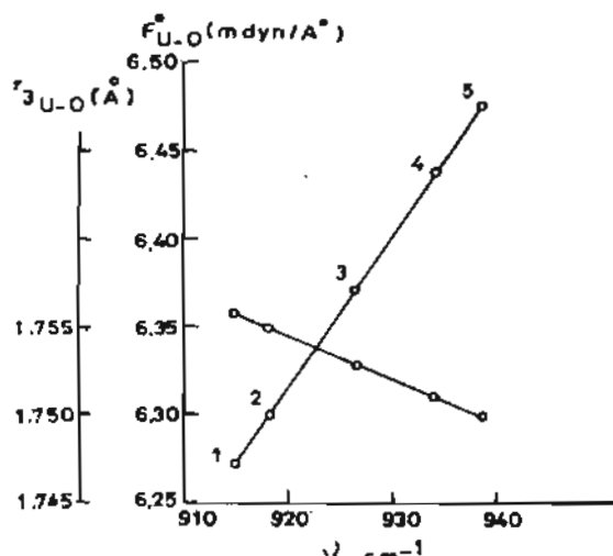
Fig. 6 The relation between r_{3U-O} (Å) and F_{U-O}^2 (mdyn Å -1 ) vs. \nu_3
