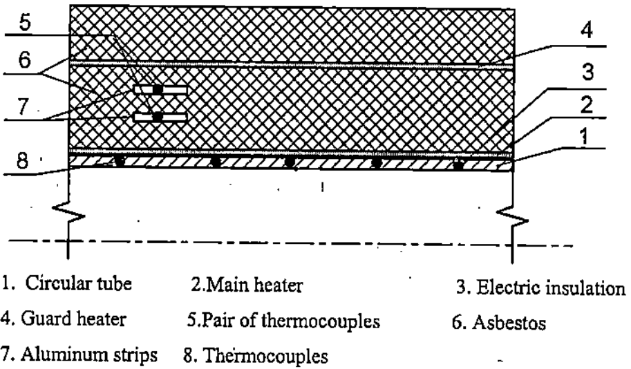
Fig.1b. Heaters arrangement
