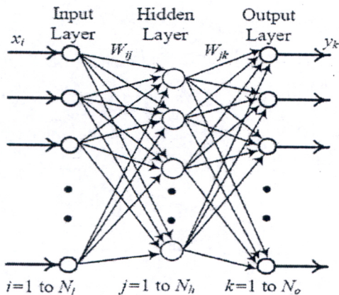
Fig. 1. Feedforward neural network [6]
