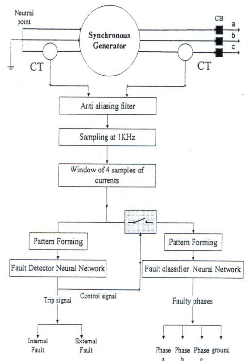
Fig.4 Schematic diagram of proposed protection algorithm
