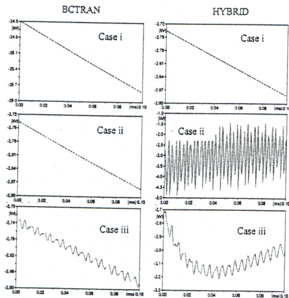
Fig. 4: Phase C Voltage of the Tested Transformer Primary side
