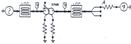
Fig. 1: EMTP/ATP Investigation System Model
