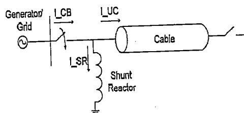
(a) A Cable-Shunt Reactor Circuit
