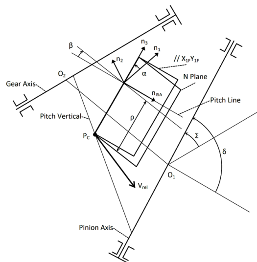
Figure 5 – N Plane and Instantaneous Screw Axis (ISA). [1, 2, 5]
