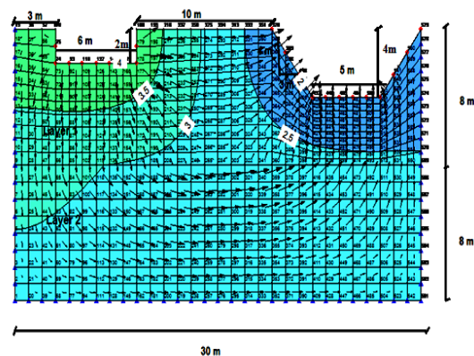
(1) Model Dimensions
