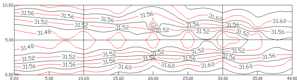
Figure 2. Contour map for the surface road
