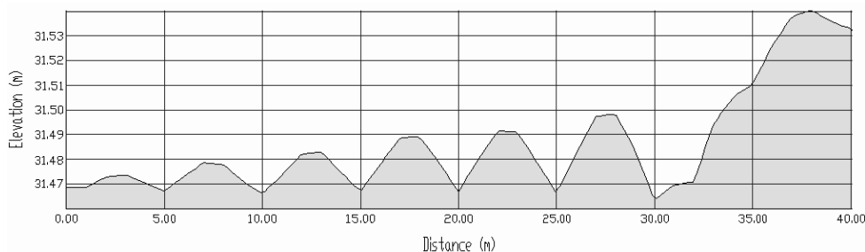
Figure 3. Longitudinal profile for the surface road
