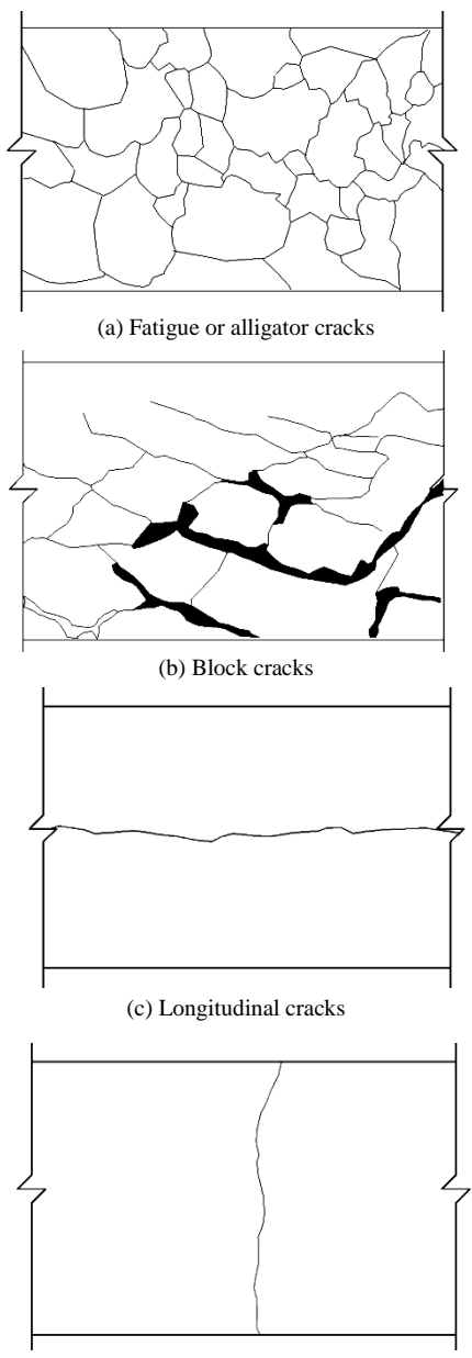
Figure 5. Pavement cracks
