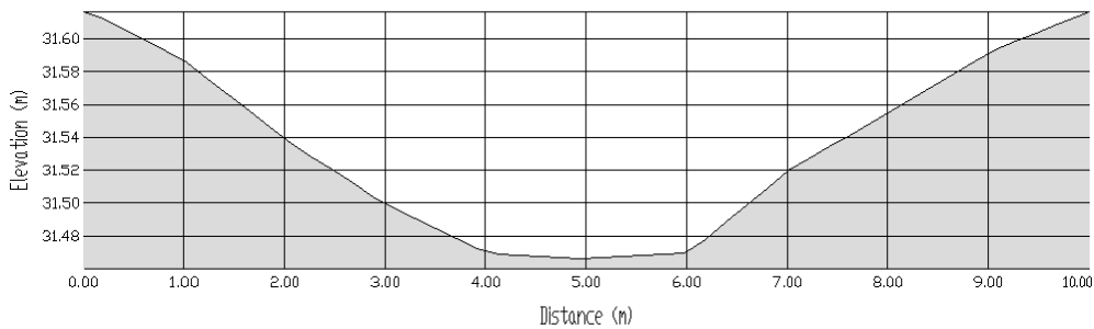
(a) Transverse profile at distance 10
