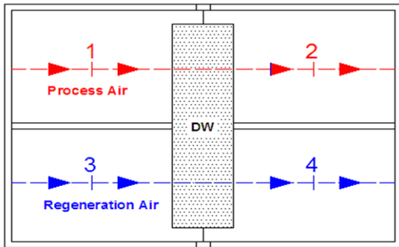
Fig. 4. Test facility section for experimental investigation of desiccant wheel.
