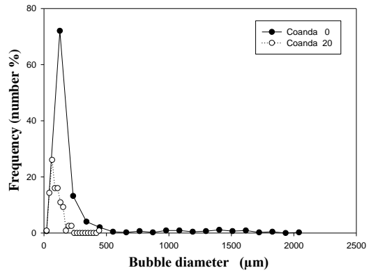
(e) Q_a = 0.9 l/min.
