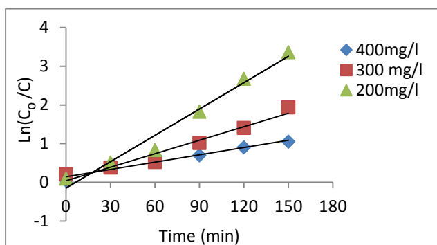
Fig. 7. Kinetics analysis of chlorpyrifos using catalyst dose= 0.25 g/L and pH=7 ± 0.5.
