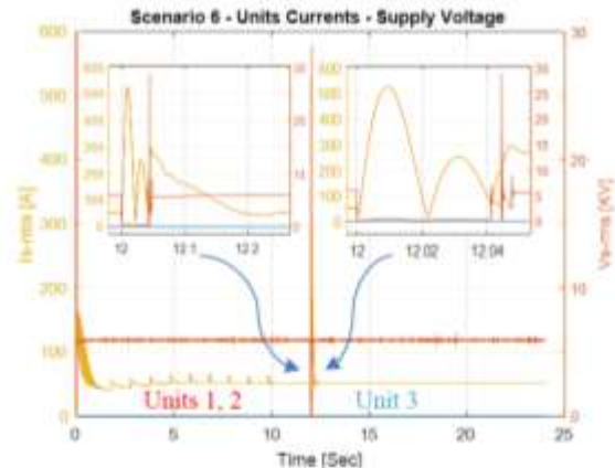
Fig. 21. The RMS plotting of line current plus the terminal (L-L) voltage for Units 1, 2 and 3 (Scenario 6).
