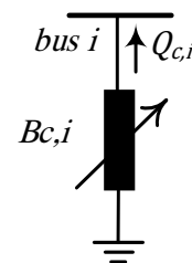
Fig. 1. capacitor bank model
