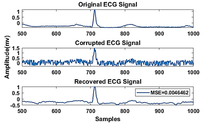
Fig. 3. Removing of EMG noise corrupted ECG signal Record101 at level SNR =15dB using the proposed SNRC system
