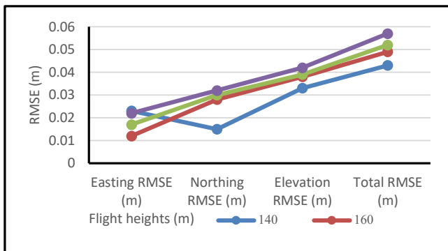
Fig. 9: The correlation between the attitude AGL and RMSE of the IG process.
